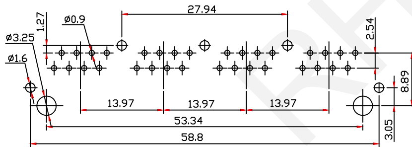
PCB Layout
